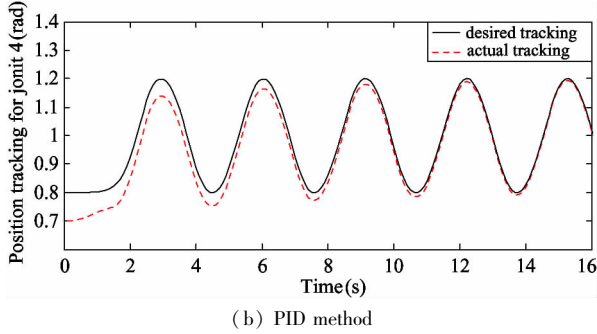
Fig. 6 Trajectory tracking control for joint 4
